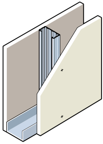
'C' STUD PARTITION SYSTEM
